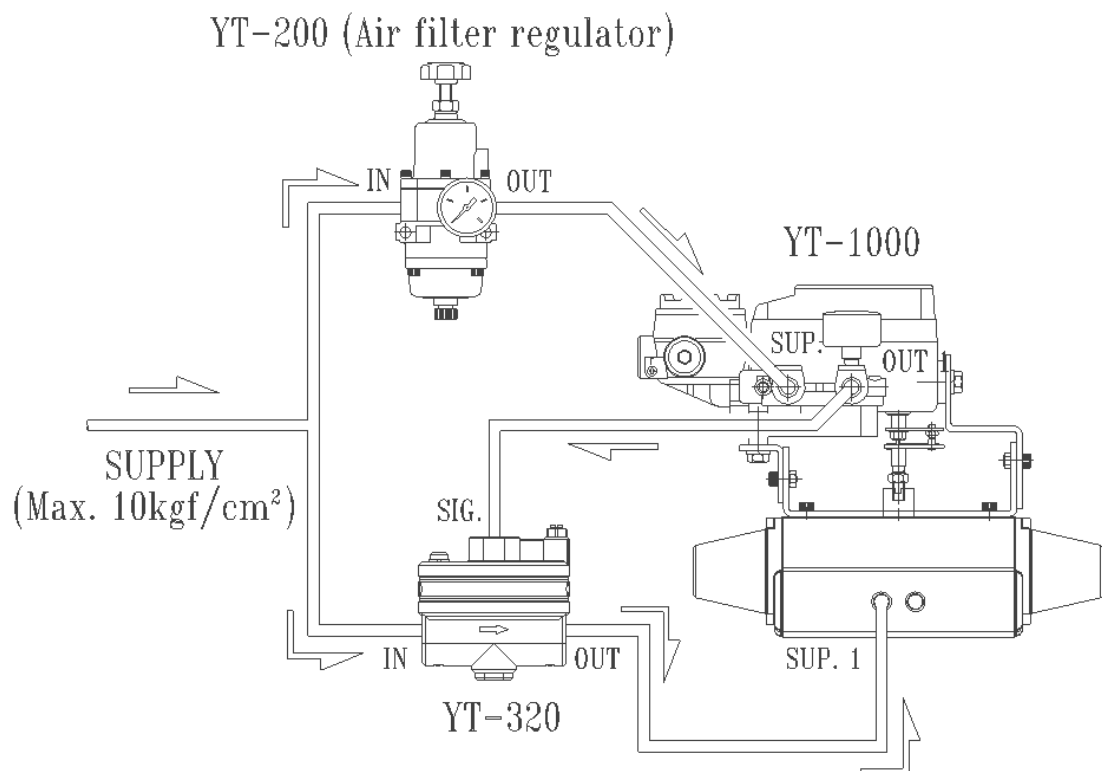
Single acting rotary actuator
