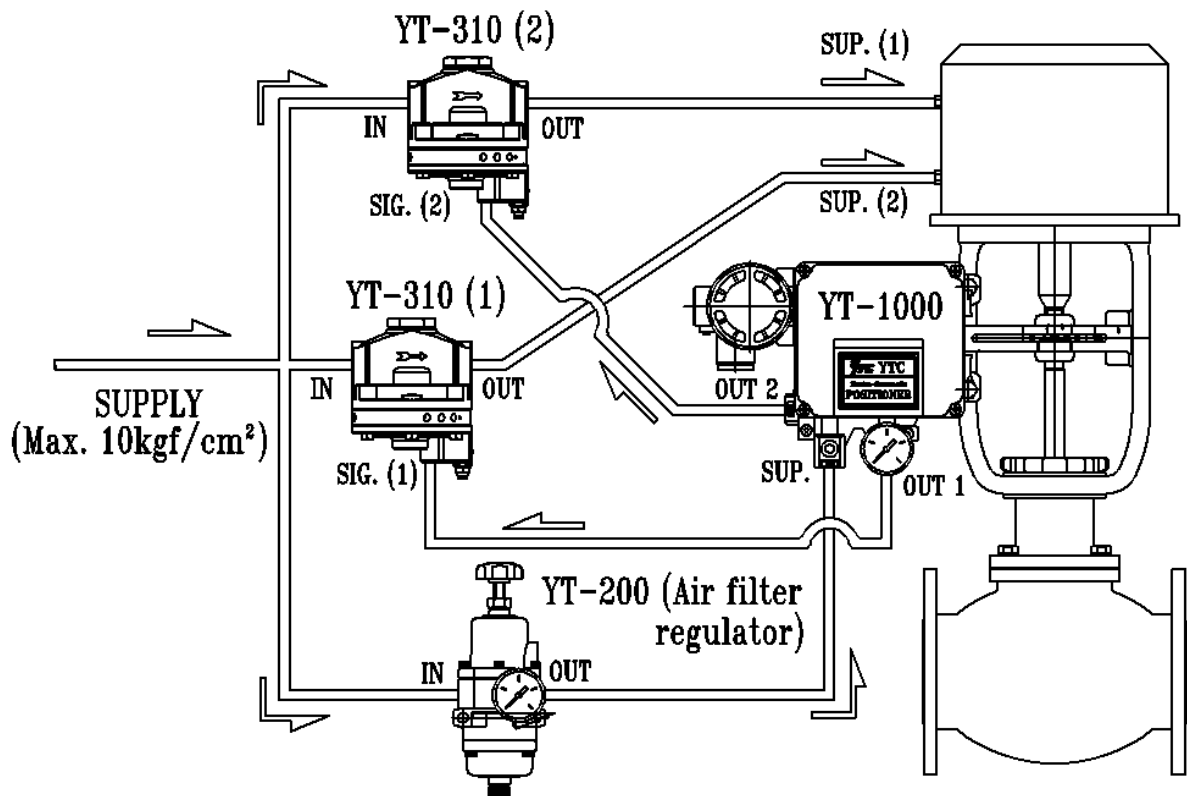
Double acting linear actuator
